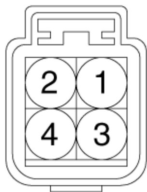
Harness Connector
